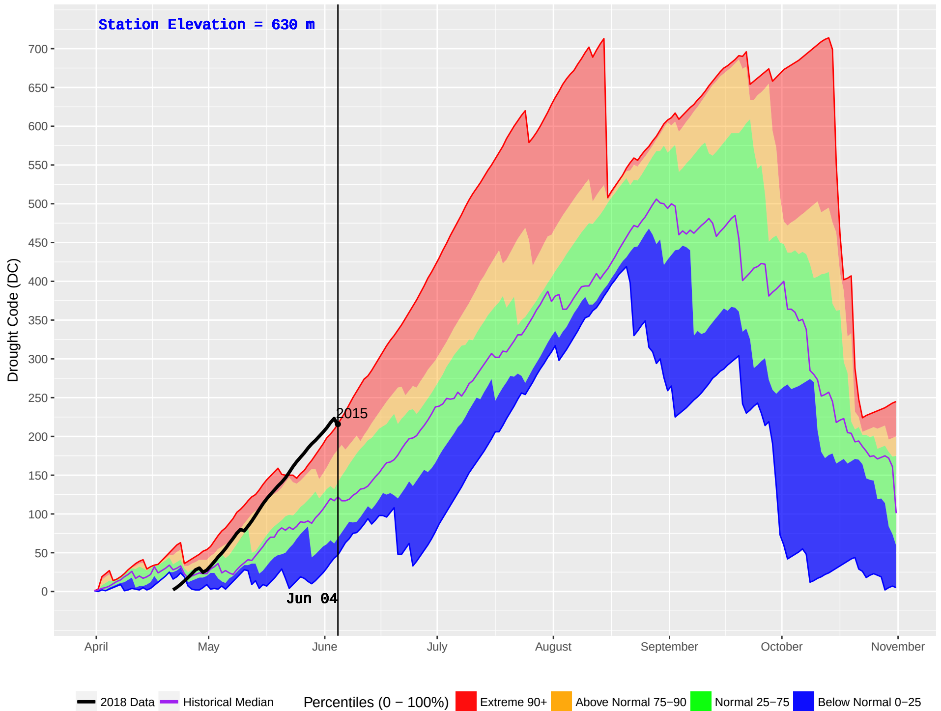
ANDERSON CREEK (977) : Historical (2007–2016) and Current (2018) Noon Drought Code (DC)
