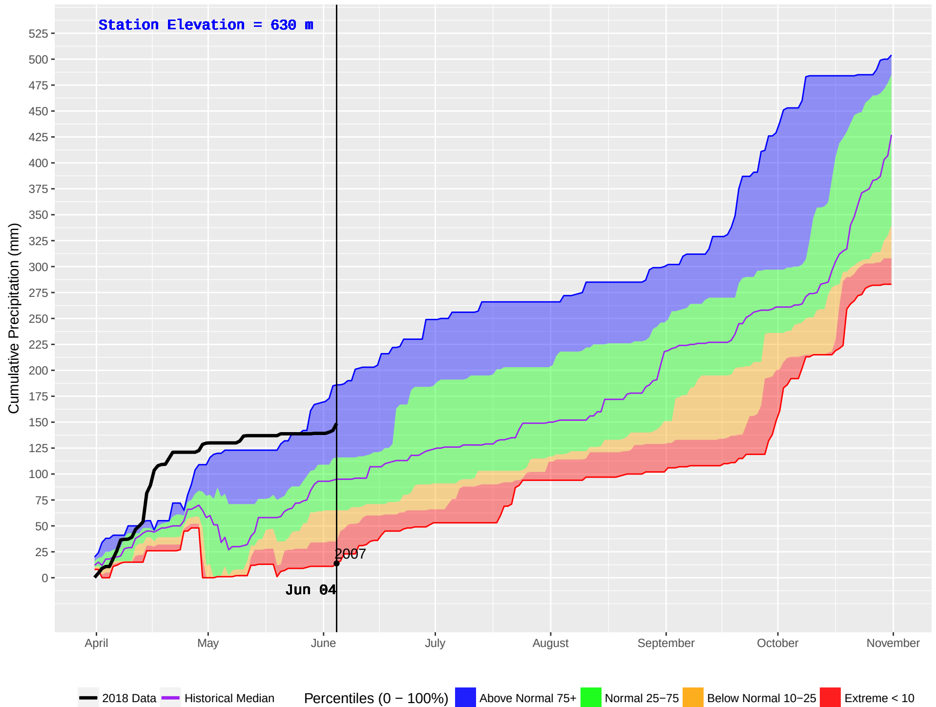
ANDERSON CREEK (977) : Historical (2007–2016) and Current (2018) Noon Cumulative Precipitation
